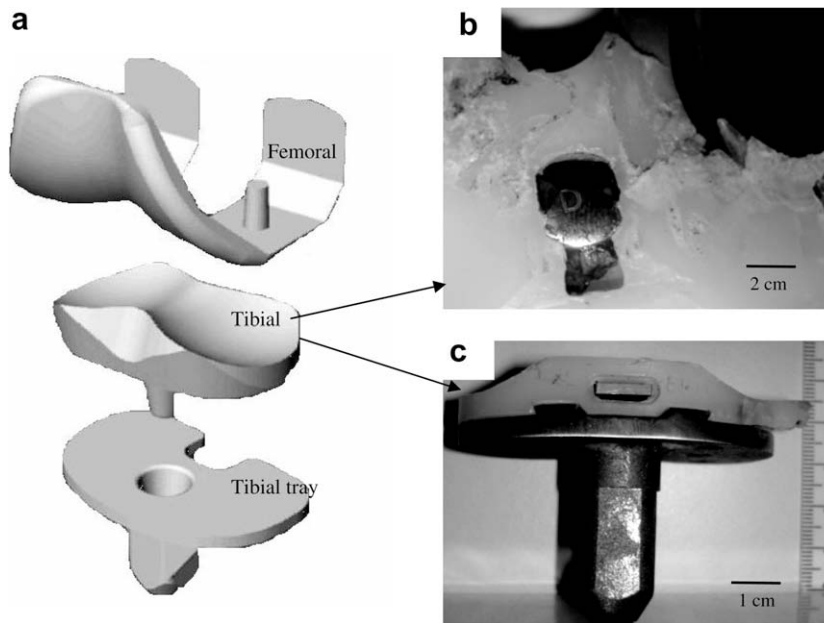
Fig. 1. Knee prosthesis: (a) schematic prosthesis components, (b) top view of the tibial base showing a severe damage and (c) front view of the tibial base.
